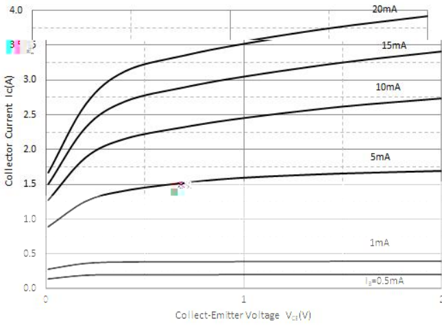
Static Characteristics
